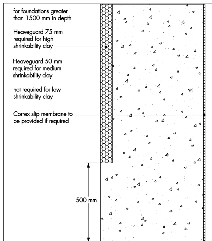
Figure 4 Detail of trench fill
