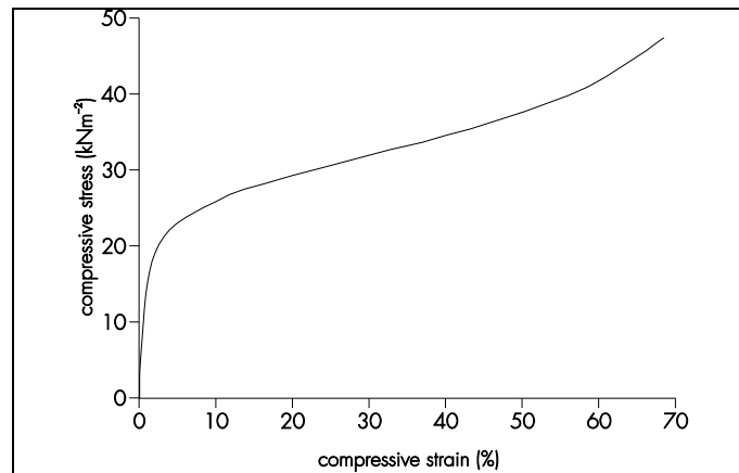
Figure 2 Compressible strain
