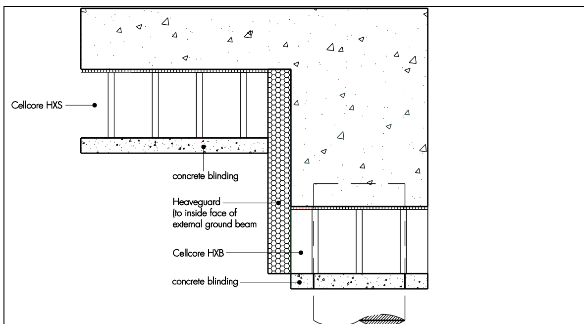
Figure 3 Detail of pile and ground beam
