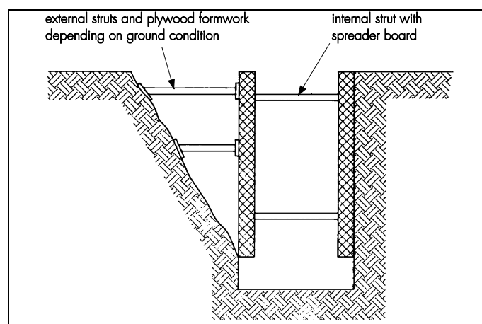
Figure 5 Typical installation
