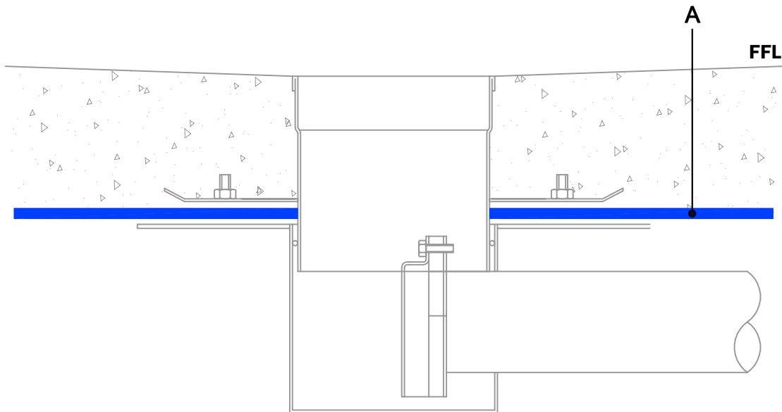
Generic Floor Gully
