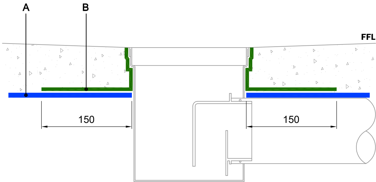
Generic Floor Gully
